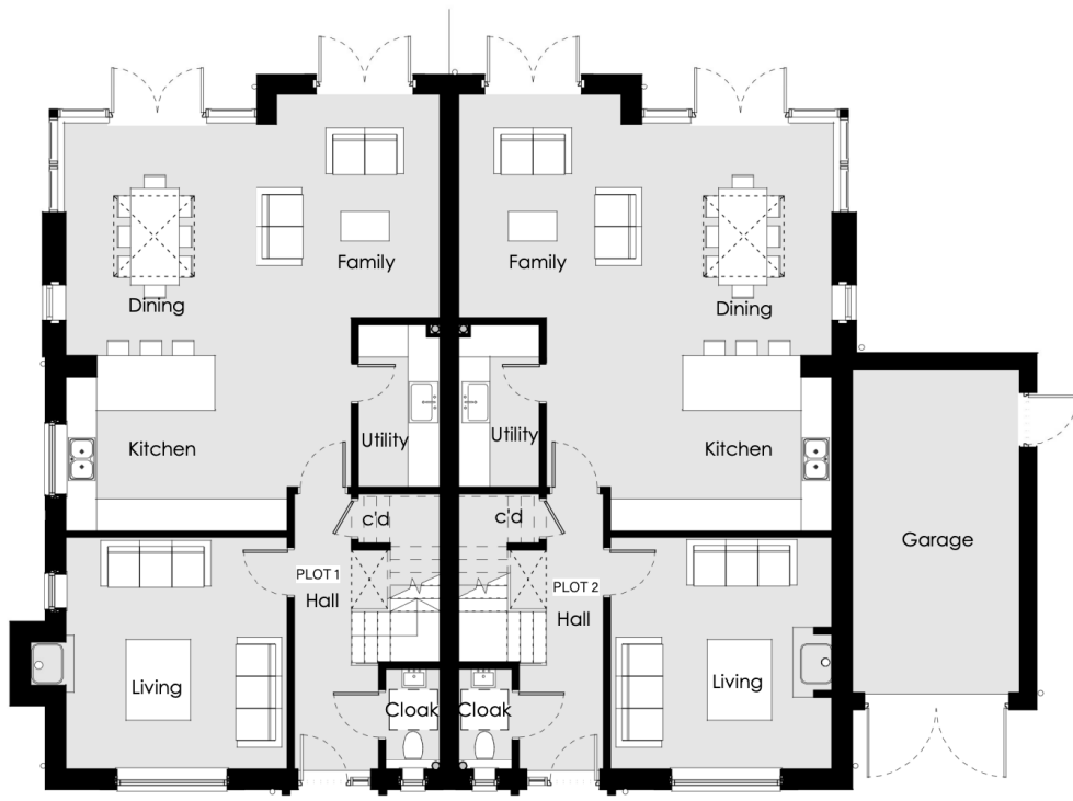
PLOT 1 GROUND FLOOR
